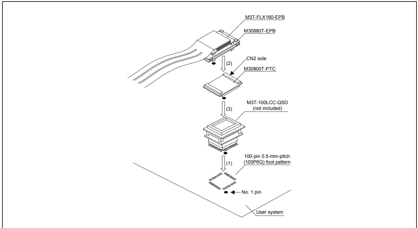
Figure 2.12 Connecting to a 100-pin 0.5-mm-pitch foot pattern (1/3)
